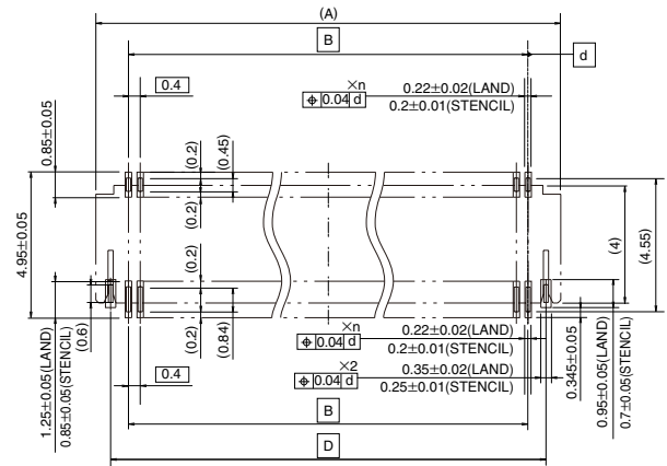
■Recommended PCB Layout and Stencil Dimensional Table
