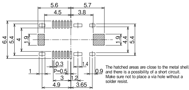
Recommended PCB Land Pattern Dimensions
