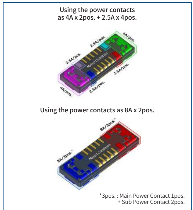
Selectable Power Contact Usage
