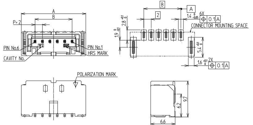
Recommended PCB Layout (t=1.6mm)
