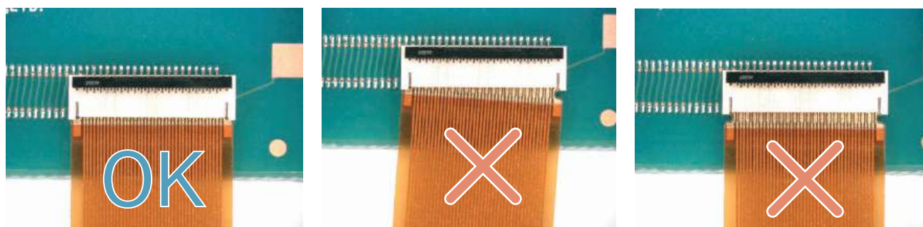
The FPC notch is hidden by the connector housing and PCB is not visible from the notch.
