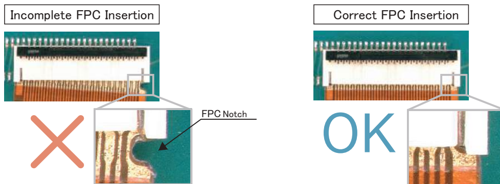
Through the FPC notch, PCB is visible.
