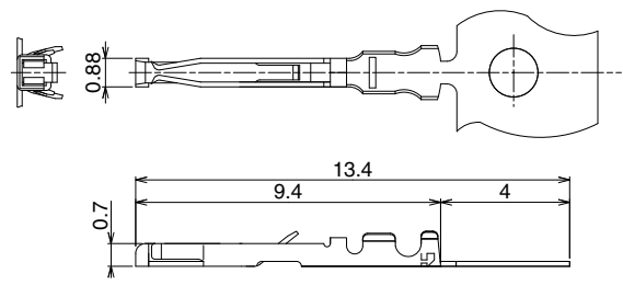
Female contact
