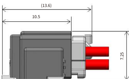
Double-row
