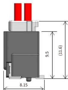
Double-row
