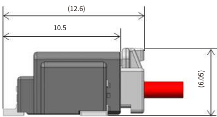
Single-row
