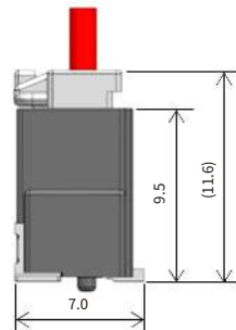
Single-row
