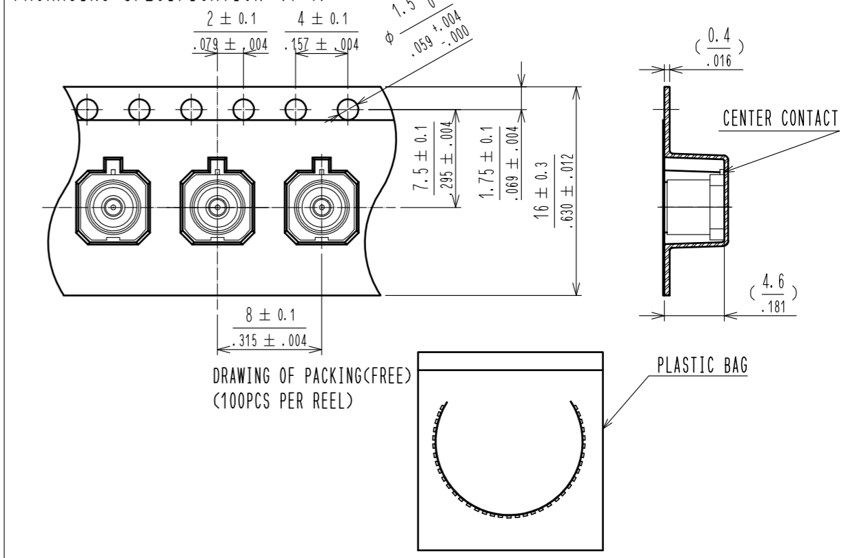
PACKAGING SPECIFICATION (4:1)
