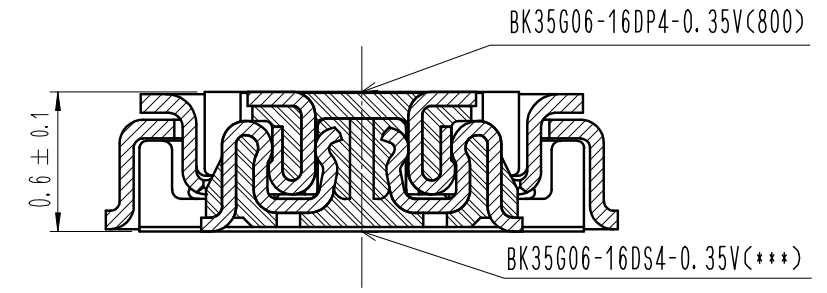
POWER CONTACT
