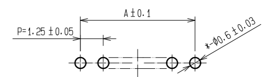
3 RECOMMENDED PATTERN (BOARD THICKNESS 1mm)
