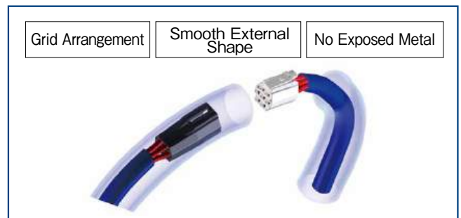
Compact shape due to 2 × 2. 2 grid layout of pins (Both are 7 contacts with 3A current rating)
