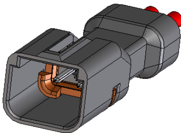
(E.g.) DF62W-2EP-2.2C +DF62W-EP2226PCF (Cables attached)
