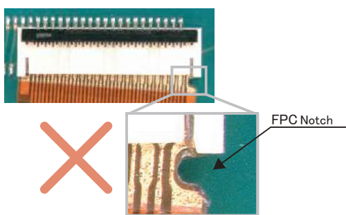
Incomplete FPC Insertion
