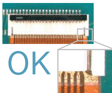
Correct FPC Insertion
