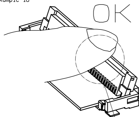
Close the actuator at the center - Correct operation -
