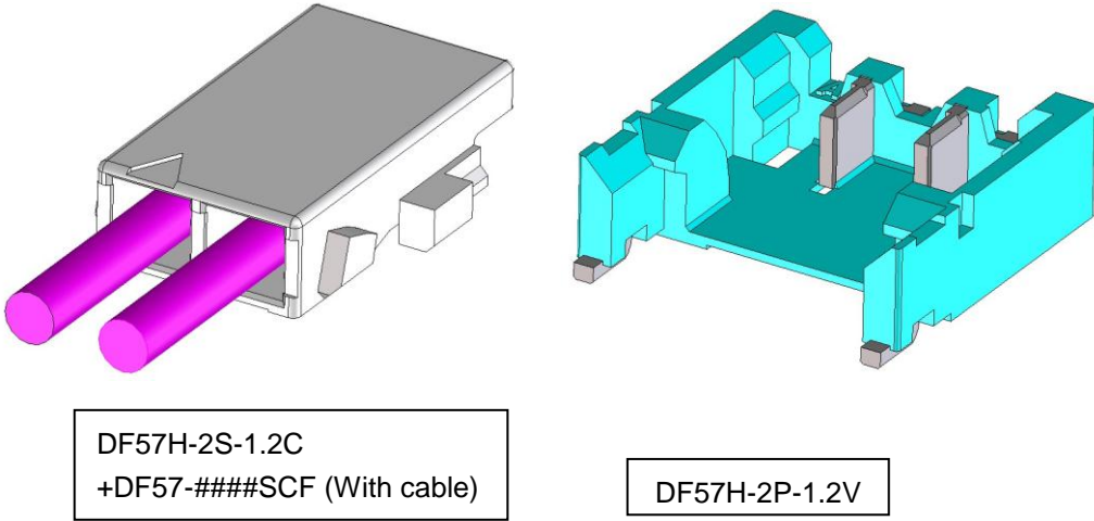
Fig. 1: DF57H Connector
