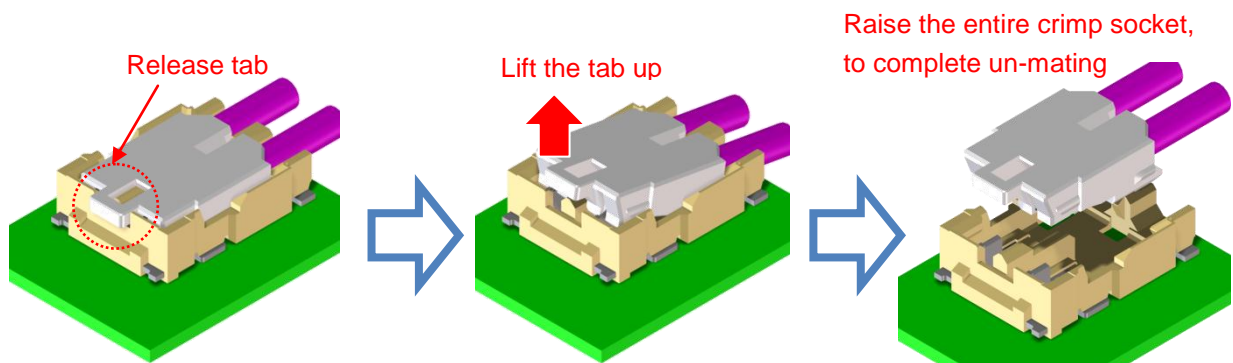
Figure 7. Unmating
