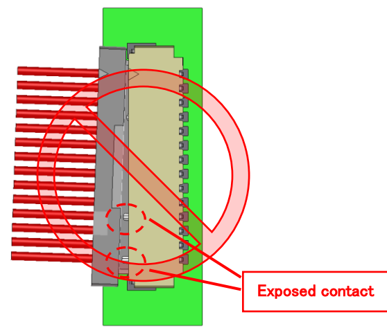
Fig.7 Incomplete mating
