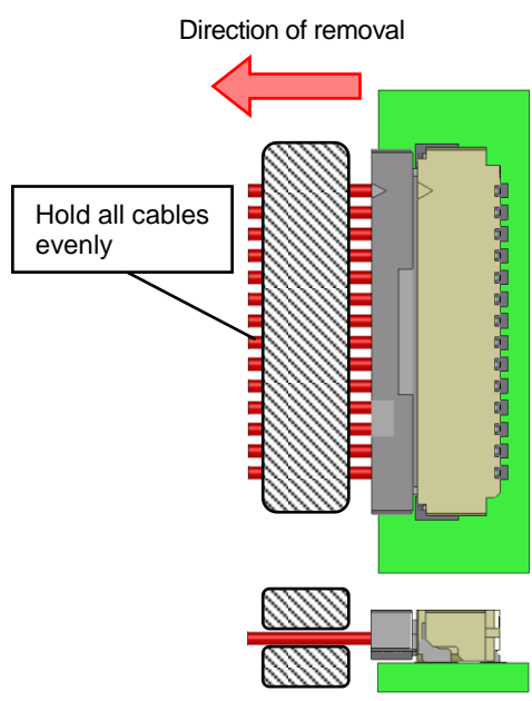
Fig.8 Removal
