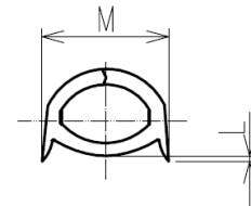
A-A (Crimp-Contact cross-section image) : where the jacket is removed.
