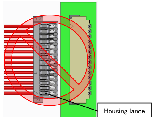
Fig.2 Reversed plug
