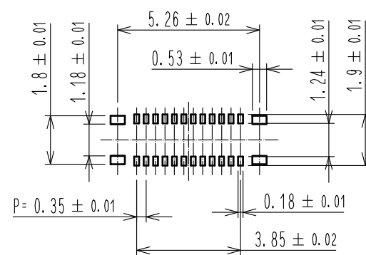
1 RECOMMENDED METAL MASK DIMENSIONS METAL MASK THICKNESS : 80 μm
