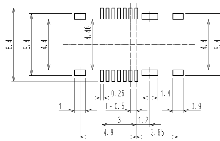
Recommended metal mask dimensions (Mask thickness : 120 μm)
