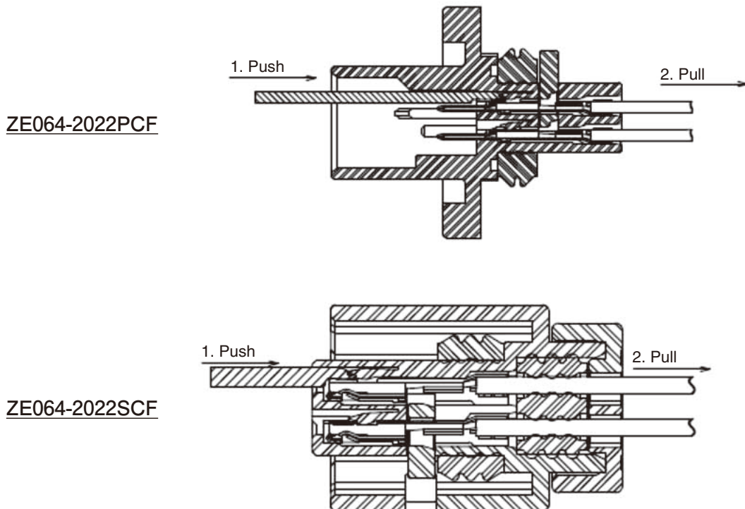
Housing Cross-Sectional Diagram
