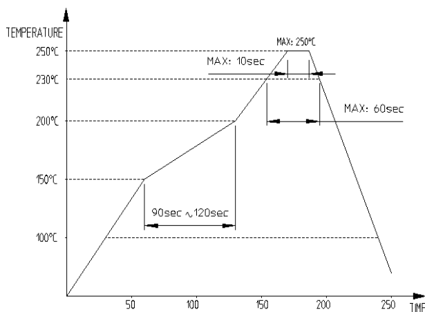
[Fig.1] REFLOW TEMPERATURE
