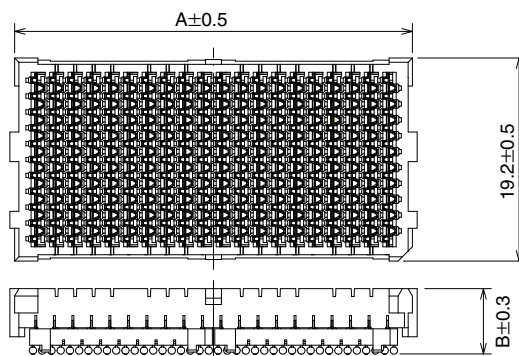
Shown : 200 position mating receptacle, IT5(H)D-200S-BGA(39)
