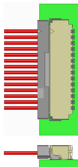
Fig.4 Insertion completed
