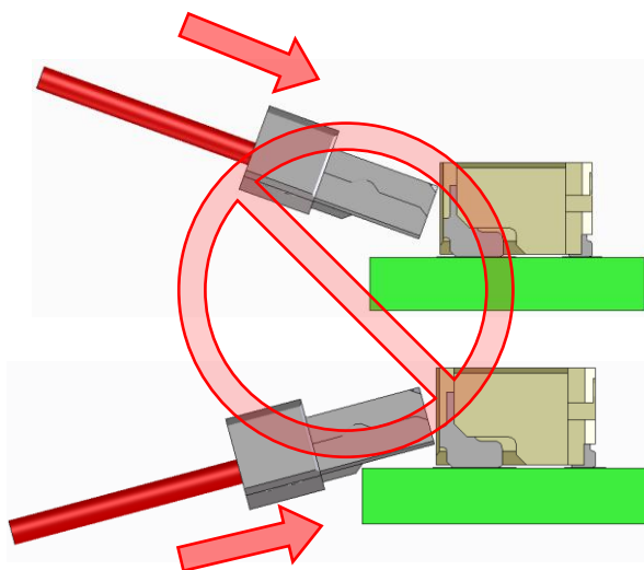
Fig.6 Prohibited insertion②
