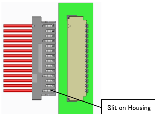
Fig.1 Correct plug orientation
