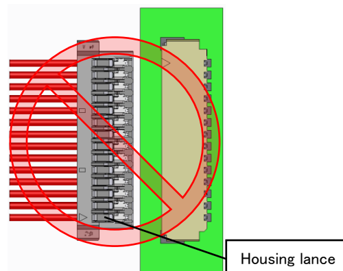
Fig.2 Reversed plug
