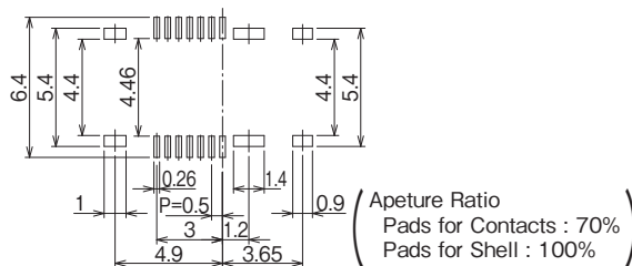
Recommended Stencil Dimensions (Stencil Thickness 120μm)
