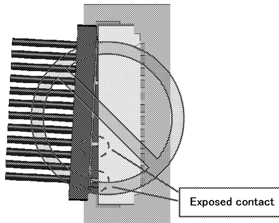
Fig.5 Incomplete mating
