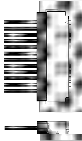
Fig.4 Insertion completed
