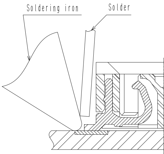
Raise of solder paste
