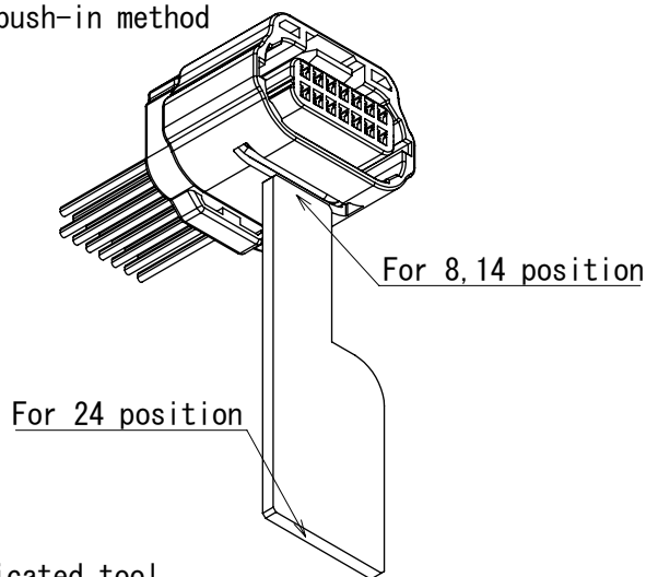
Dedicated tool appearance and dimentions (mm)
