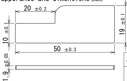
Dedicated tool appearance and dimentions (mm)
