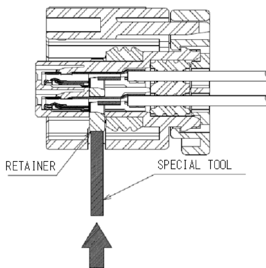
Connector cross section
