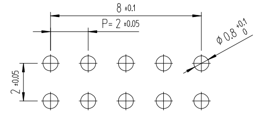
RECOMMENDED LAND PATTERN (FREE) (PCB THICKNESS t=1.6mm)
