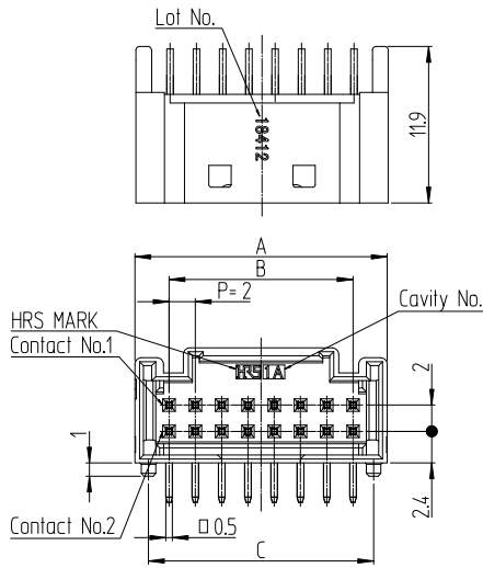
*The above drawing is of guide-boss type.
