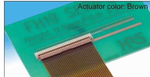
FH19SC – FPC/FFC thickness : 0.3 \pm 0.03 mm
