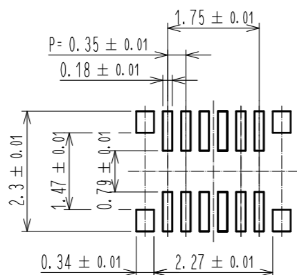
RECOMMENDED METAL MASK DIMENSIONS (10:1) \triangle METAL MASK THICKNESS : 80 \mu m
