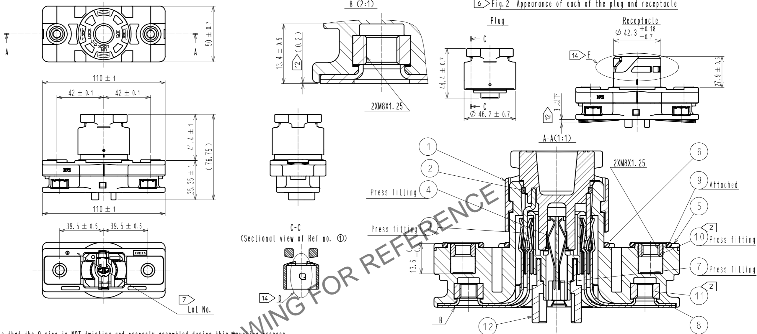
6 Fig.2 Appearance of each of the plug and receptacle
