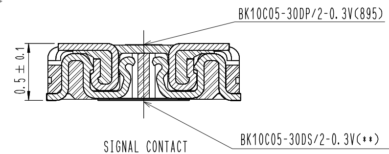
ENGAGEMENT FIGURE (30:1)
