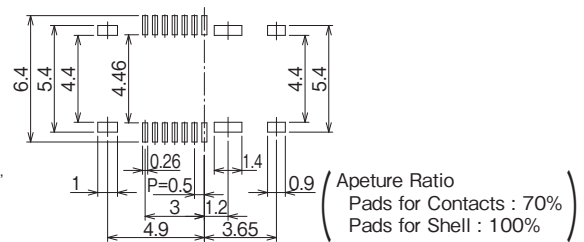
Recommended Stencil Dimensions (Stencil Thickness 120μm)
