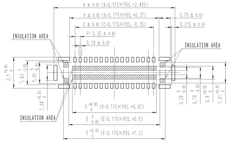
Receptacle side recommended PWB pattern
