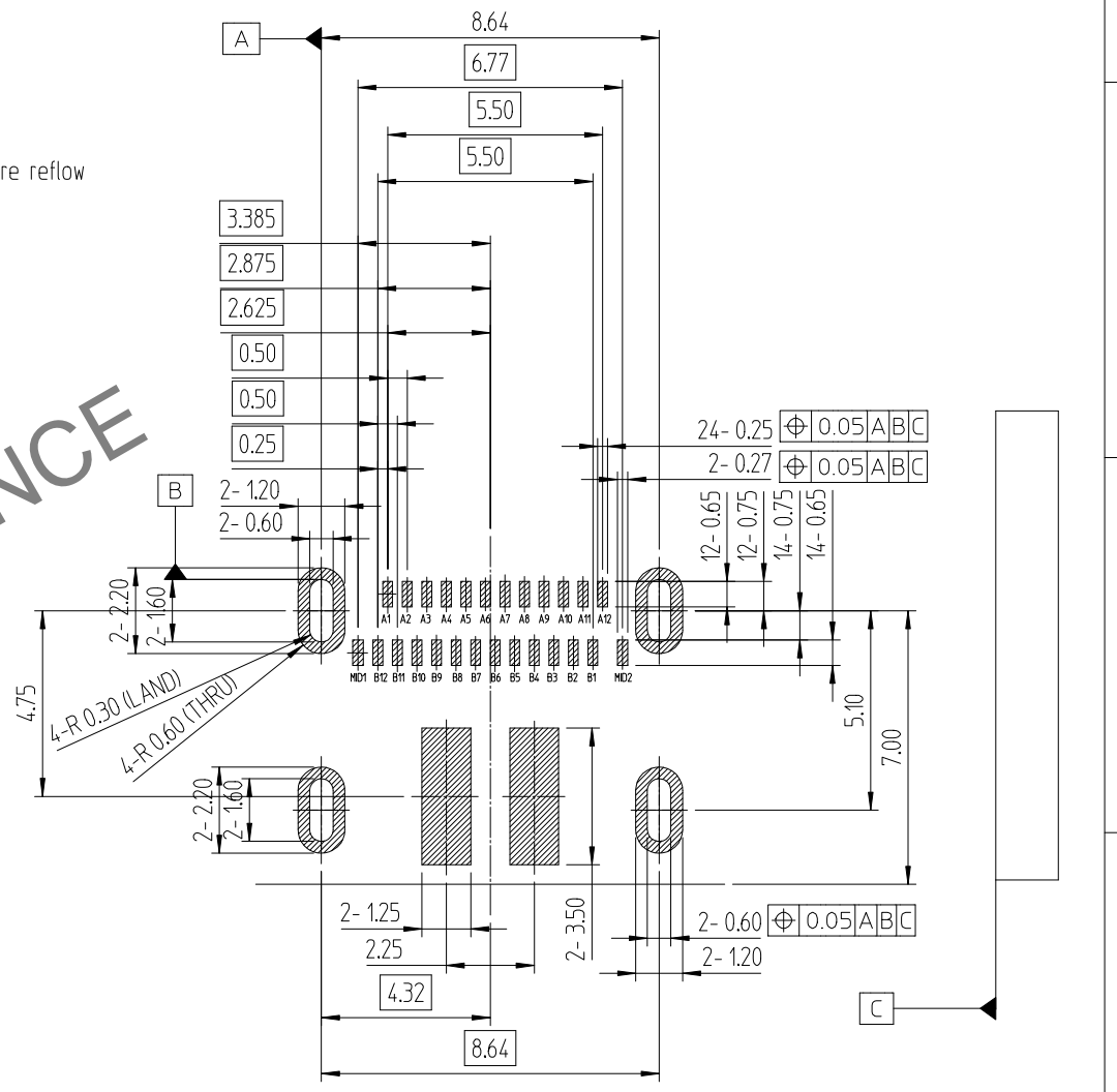
RECOMMENDED PCB LAY OUT (TOP-VIEW) (GENERAL TOLERANCE : ±0.05)
