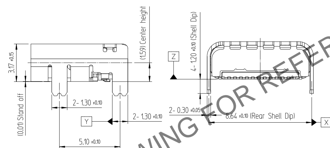
PCB MOUNTING POSITION
