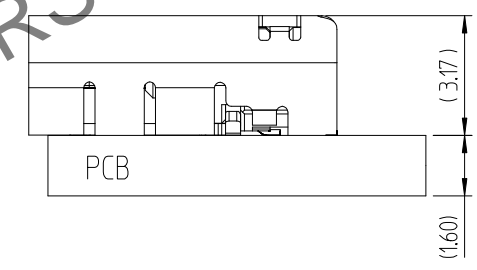
PCB MOUNTING POSITION
