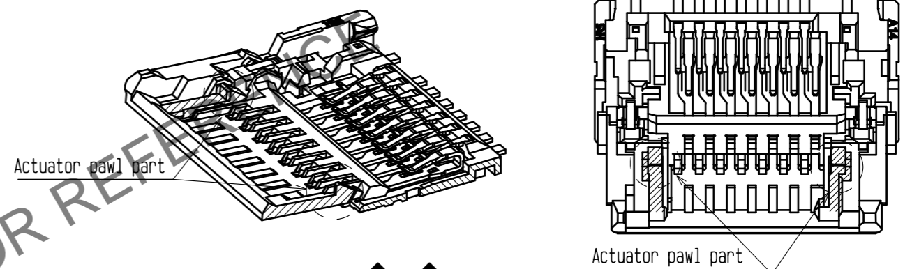
Example 24) Section - locking area -
