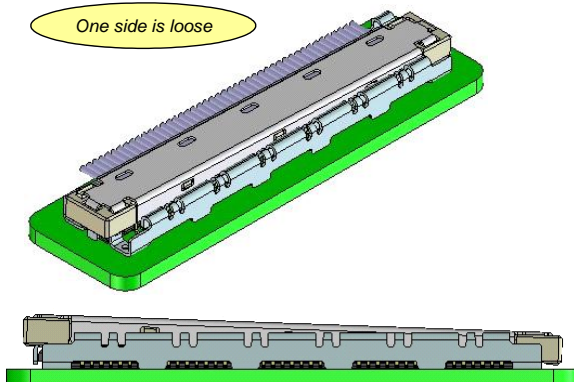
Mated aslant
