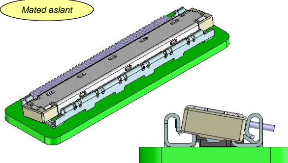
Mated aslant
